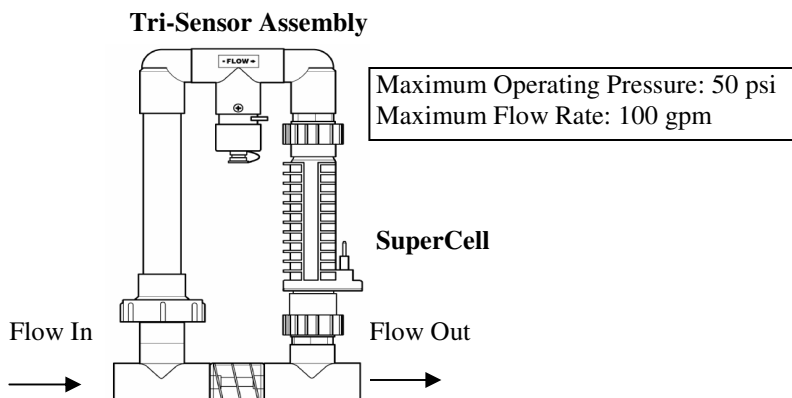
Patented Automatic Flow Bypass Manifold Assembly
